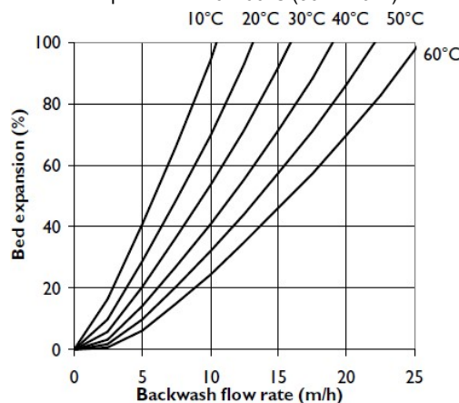
Figure 1: Backwash Expansion
