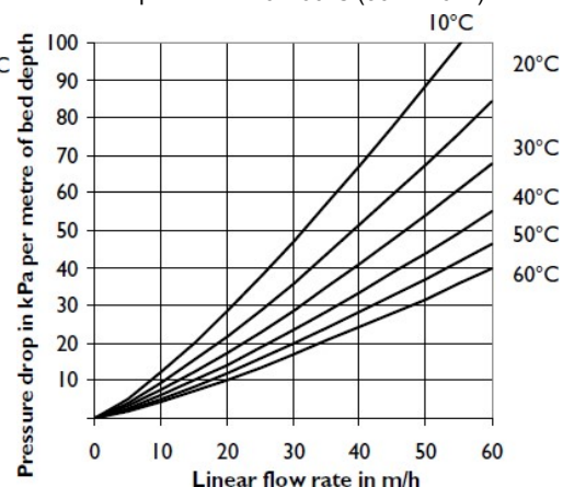
Figure 2: Pressure Drop
