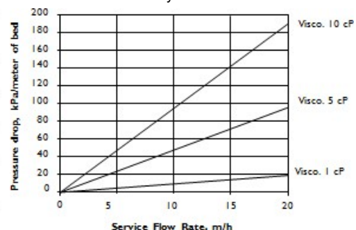
Figure 2: Pressure Drop
