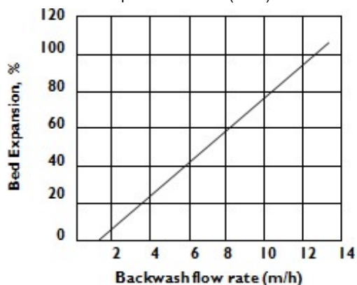
Figure 1: Backwash Expansion
