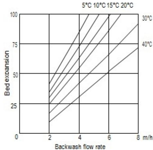
Figure 1: Backwash Expansion
