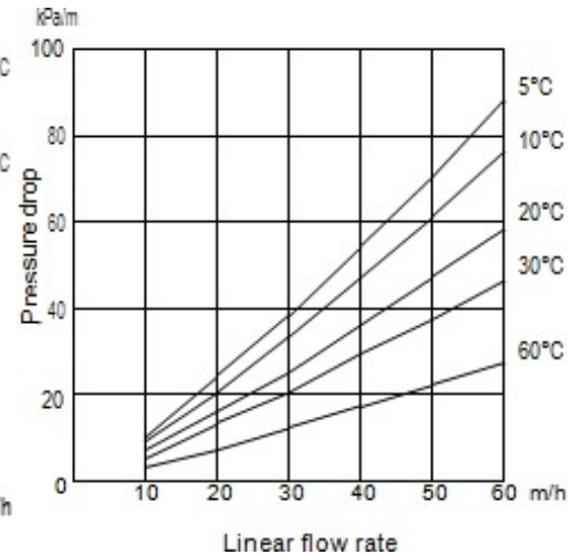
Figure 2: Pressure Drop
