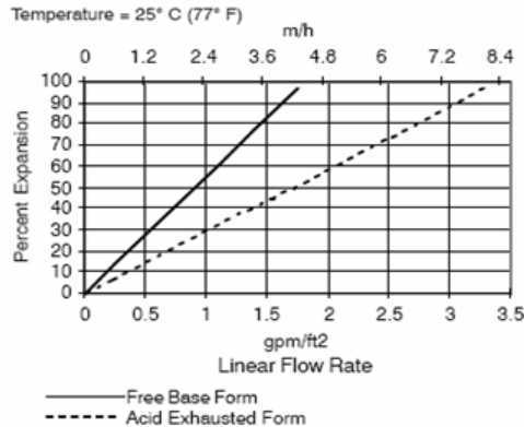
Figure 1: Backwash Expansion
