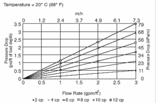
Figure 2: Pressure Drop
