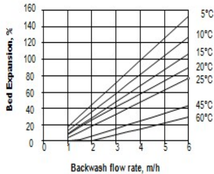
Figure 1: Backwash Expansion Temperature = 5 – 60°C (41 – 140°F)
