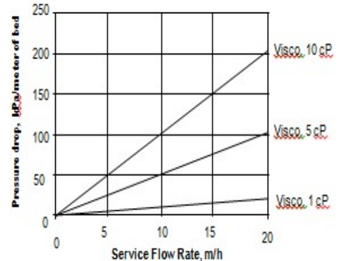
Figure 2: Pressure Drop Viscosity = 1 – 10 cP
